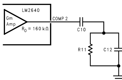
Figure 21. Typical Compensation Network
