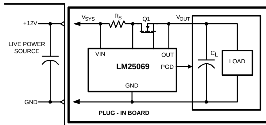
Figure 22. LM25069 Application
