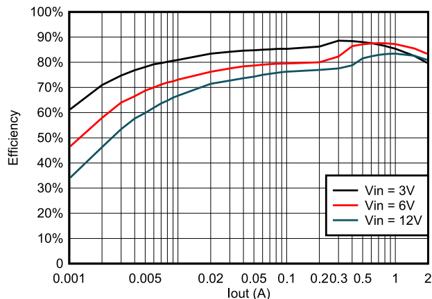
Figure 6-7. Efficiency at 0.8 V_{OUT} with a 1- \mu\text{H} Inductor
