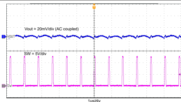
Figure 8-7. Output Voltage Ripple with 2-A Loading
