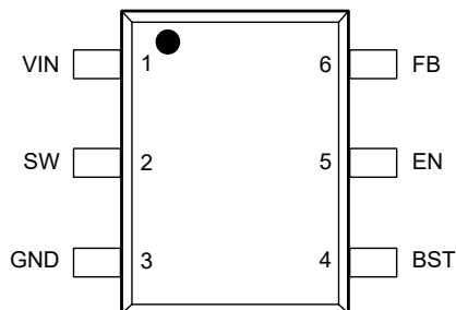
Figure 5-1. 6-Pin SOT563 DRL Package (Top View)
