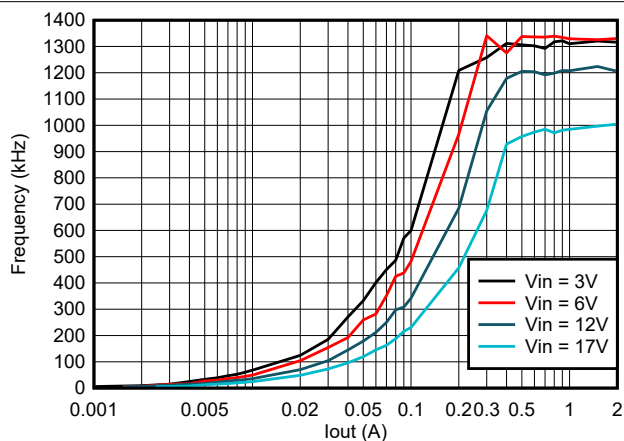
Figure 8-3. Frequency vs Loading
