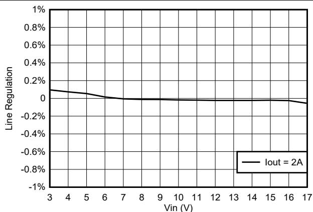
Figure 8-5. Line Regulation vs V_{IN}
