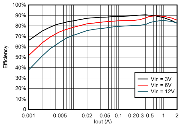
Figure 6-8. Efficiency at 1.05 V_{OUT} with a 1.2- \mu\text{H} Inductor
