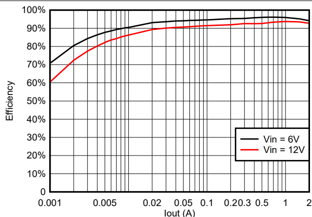
Figure 6-9. Efficiency at 3.3 V_{OUT} with a 2.2- \mu\text{H} Inductor
