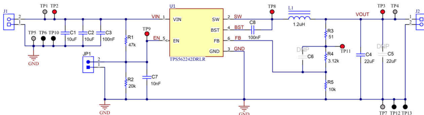
Figure 8-1. Schematic
