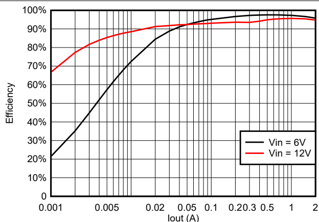
Figure 6-10. Efficiency at 5 V_{OUT} with a 3.3- \mu\text{H} Inductor
