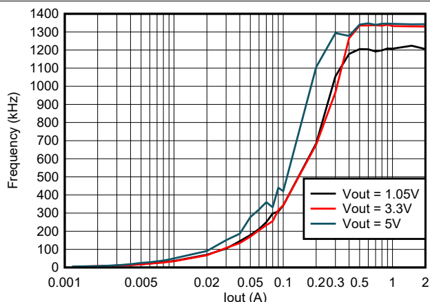
Figure 6-12. Frequency vs Loading, V_{IN} = 12\text{ V}
