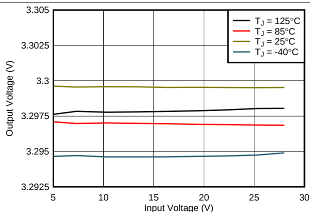
Figure 2. 3.3-V Line Regulation vs V_{IN} and Temperature
