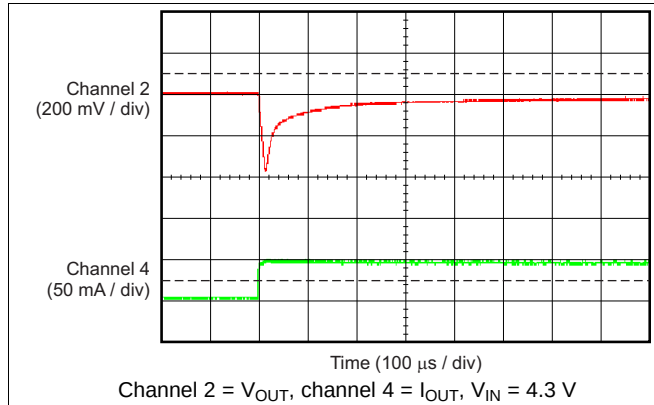
Figure 31. TPS70933-Q1 Load Transient (0 mA to 50 mA)
