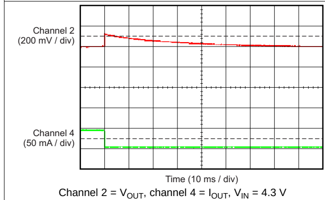
Figure 33. TPS70933-Q1 Load Transient (50 mA to 0 mA)
