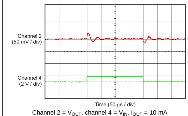
Figure 35. TPS70912-Q1 Line Transient (2.7 V to 3.7 V)
