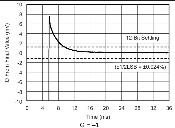
Figure 22. Large-Signal Settling Time (10-V Positive Step)
