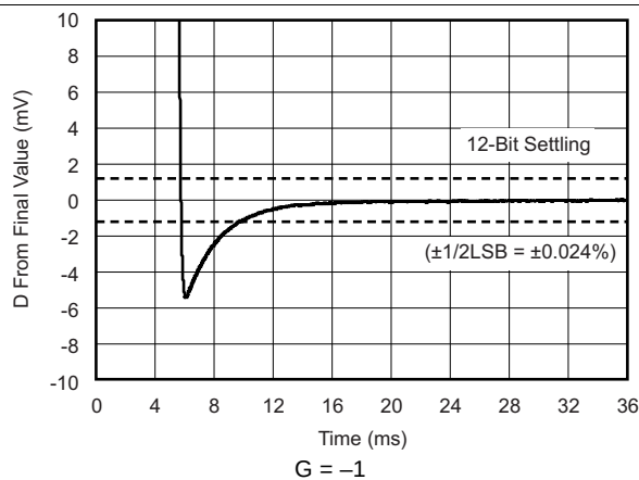
Figure 23. Large-Signal Settling Time (10-V Negative Step)
