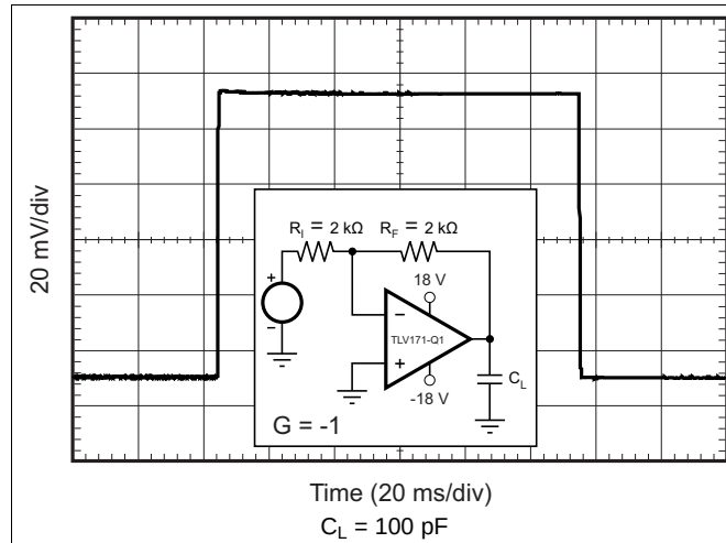
Figure 19. Small-Signal Step Response (100 mV)
