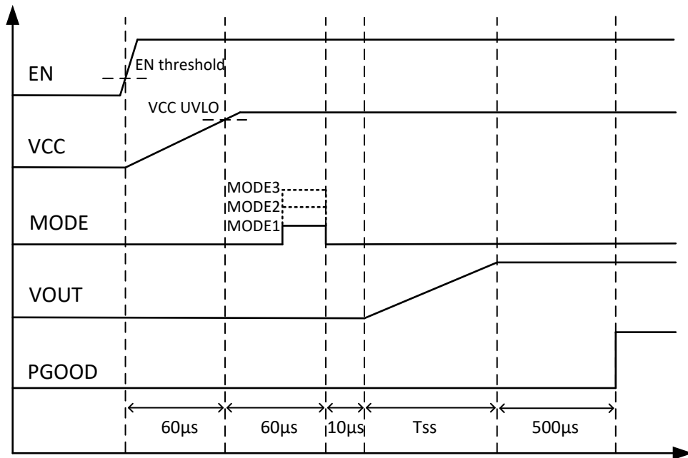
Figure 18. Start-Up Sequence
