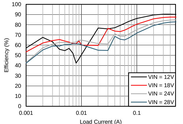
Figure 66. Efficiency
