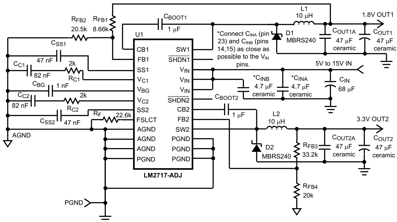
Figure 22. 3.3V, 1.8V Output Application
