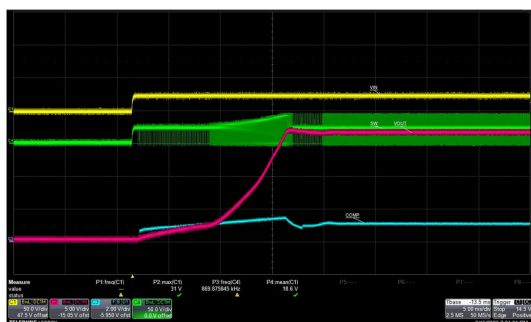
V_{IN} stepped to 24 V 0-A Load
