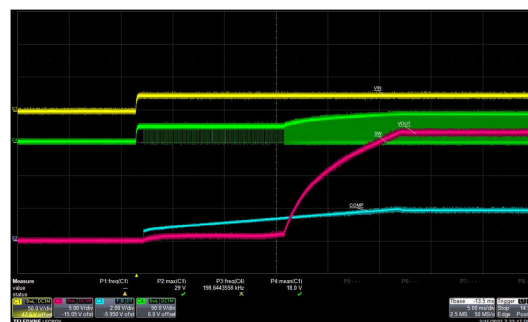
V_{IN} stepped to 24 V 1-A Load
