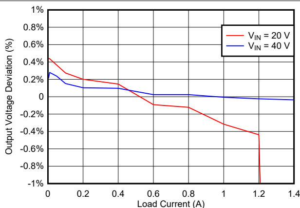
Figure 8-3. Load Regulation
