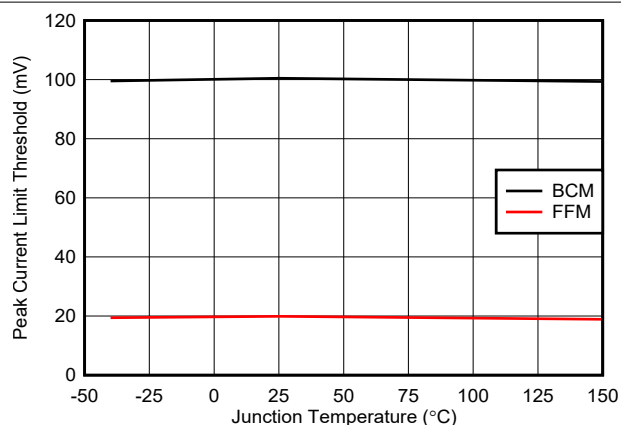
Figure 6-10. Peak Current Limit Thresholds vs. Temperature
