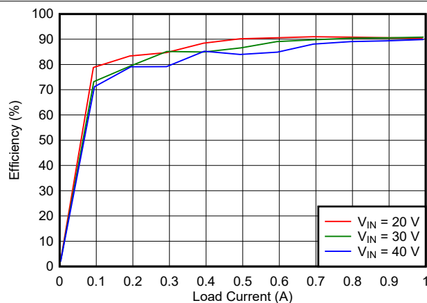
Figure 8-2. Efficiency
