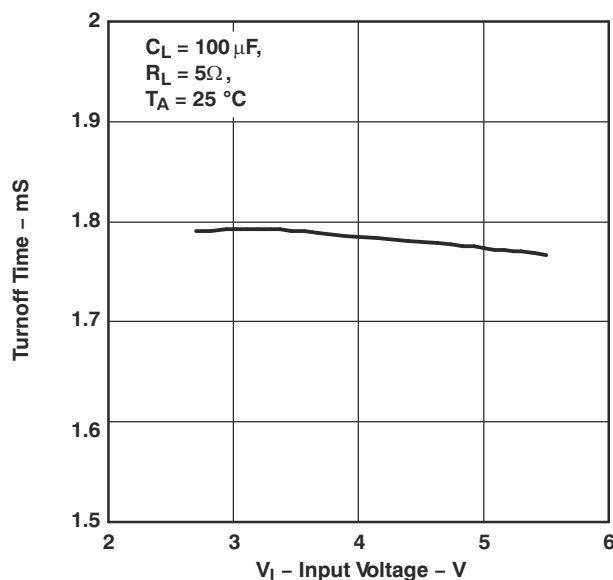
Figure 5-2. Turnoff Time vs Input Voltage
