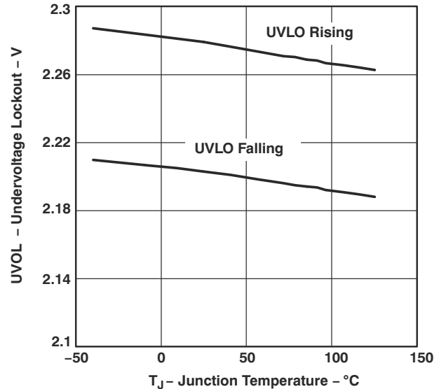
Figure 5-10. Undervoltage Lockout vs Junction Temperature
