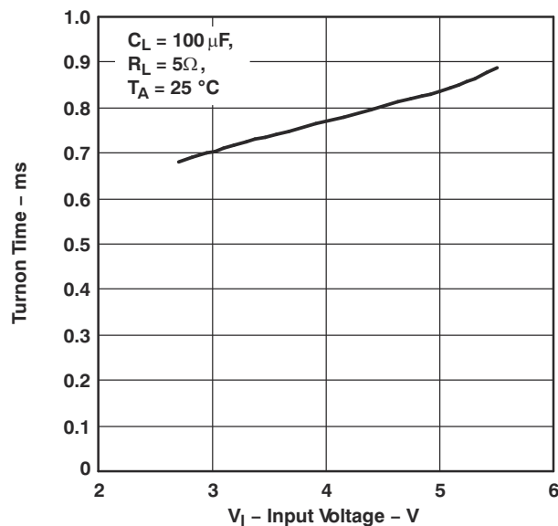
Figure 5-1. Turnon Time vs Input Voltage
