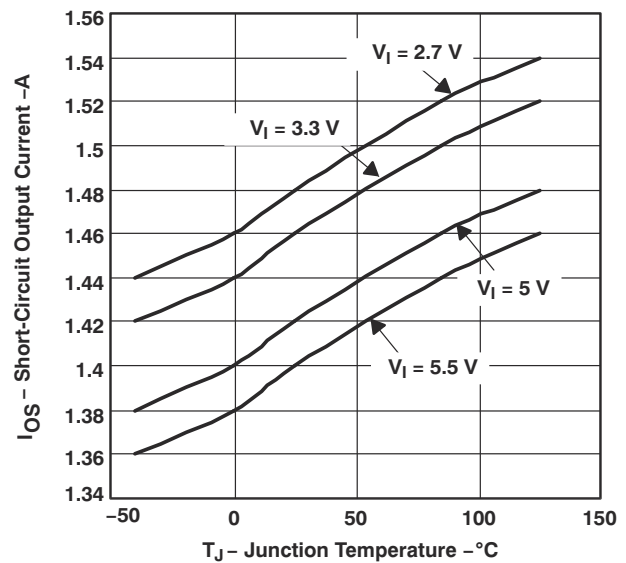
Figure 5-8. Short-Circuit Output Current vs Junction Temperature
