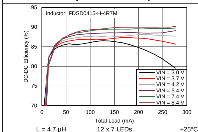
Figure 12. Boost Efficiency
