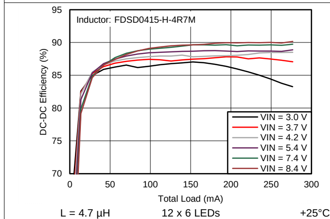
Figure 10. Boost Efficiency
