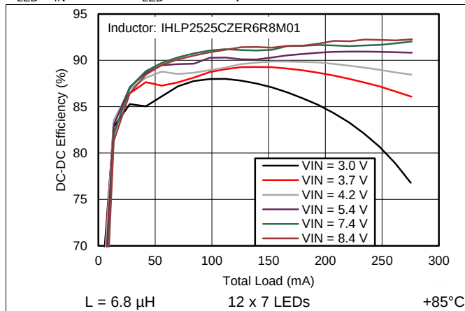
Figure 8. Boost Efficiency
