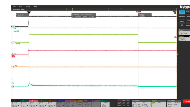
Figure 5-7. Power Up into Short-Circuit Protection
