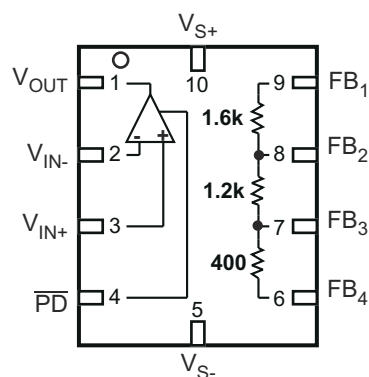
Figure 6-2. OPA836 RUN Package 10-Pin WQFN Top View
