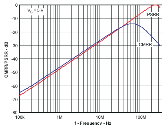
Figure 7-44. Common-Mode/Power Supply Rejection Ratios vs Frequency
