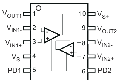
Figure 6-5. OPA2836 DGS Package 10-Pin VSSOP Top View
