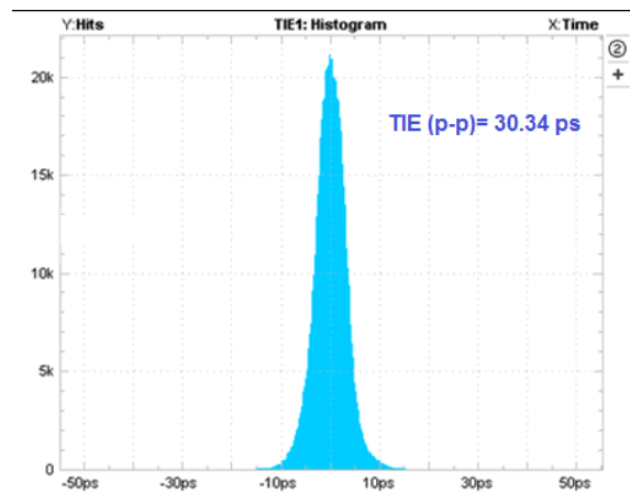
Figure 7-3. Time Interval Error Histogram: 2.25 Gbps With No Device
