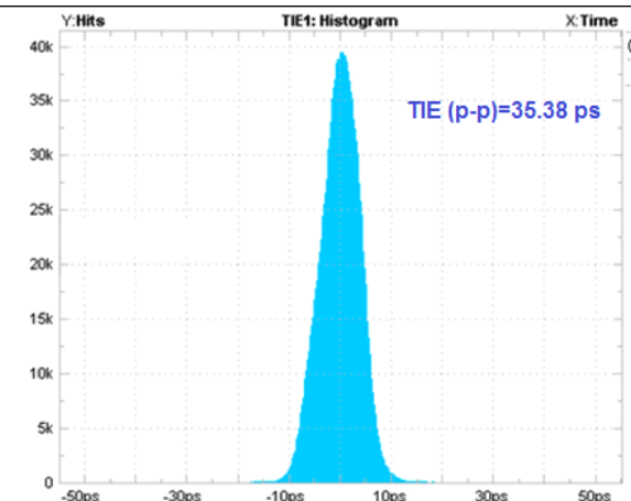
Figure 7-5. Time Interval Error Histogram: 2.25 Gbps With TS3USB3031 (Added Jitter = 5.04 ps)
