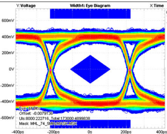
Figure 7-4. Eye Pattern Error Histogram: 2.25 Gbps With TS3USB3031 (Added Jitter = 5.04 ps)
