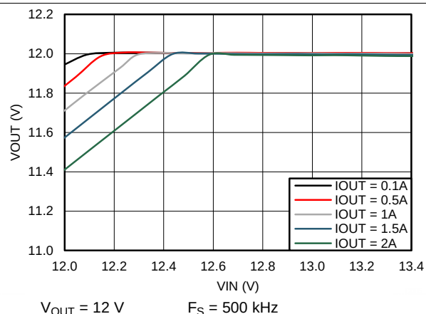
Figure 74. Dropout Curve
