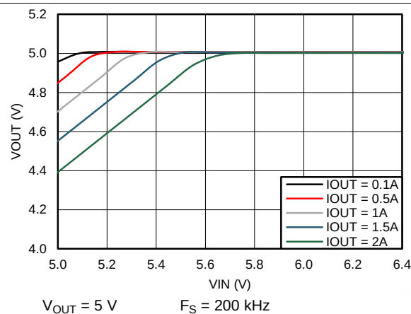
Figure 62. Dropout Curve
