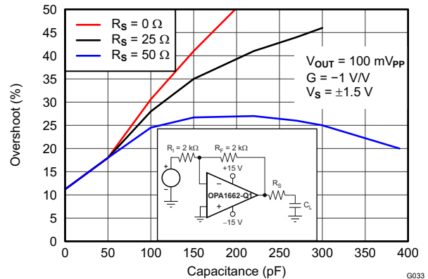
Figure 28. Small-Signal Overshoot vs Capacitive Load
