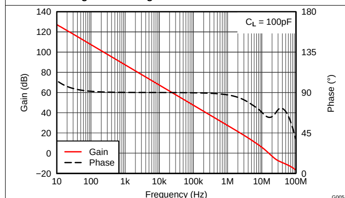
Figure 5. Gain and Phase vs Frequency
