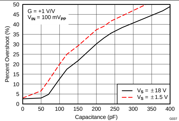
Figure 30. Percent Overshoot vs Capacitive Load
