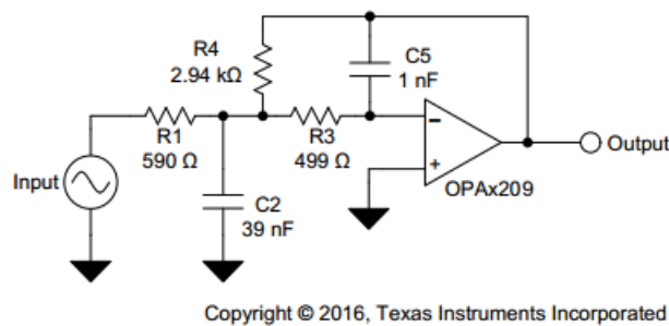
Figure 35. Low-Pass Filter
