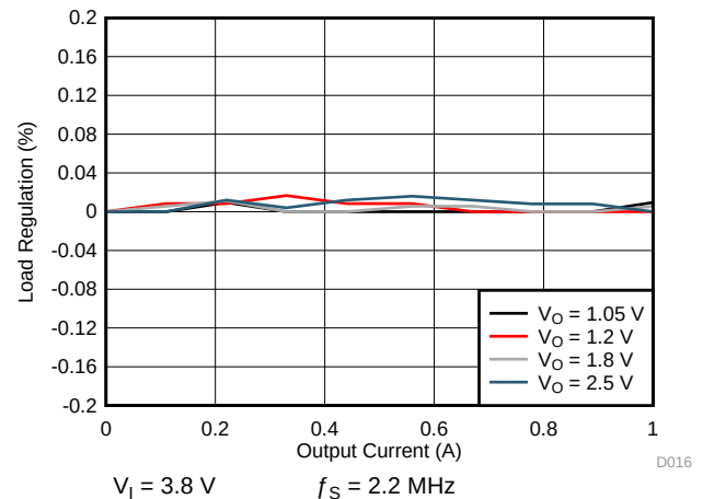
Figure 7-12. SMPS Load Regulation for 1-A Single Phase
