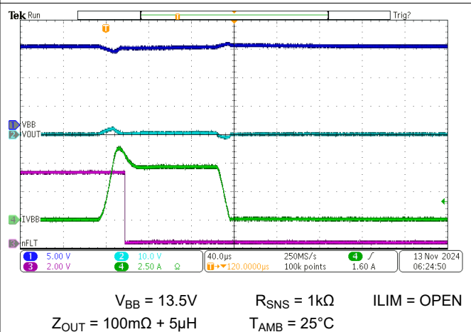
Figure 6-16. Permanent Short Behavior With ILIM Open
