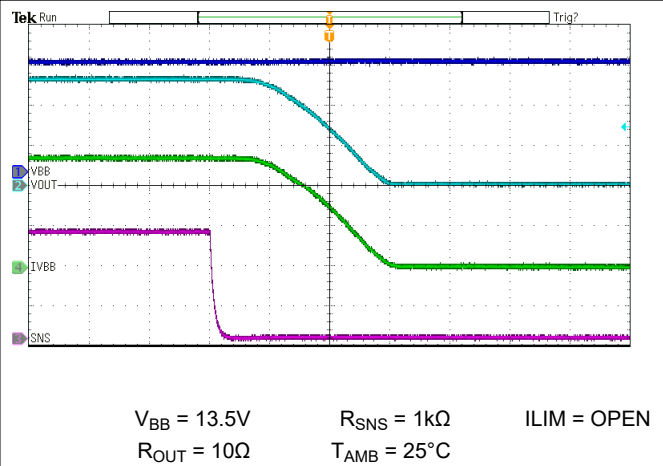
Figure 6-14. Switch Turn-Off
