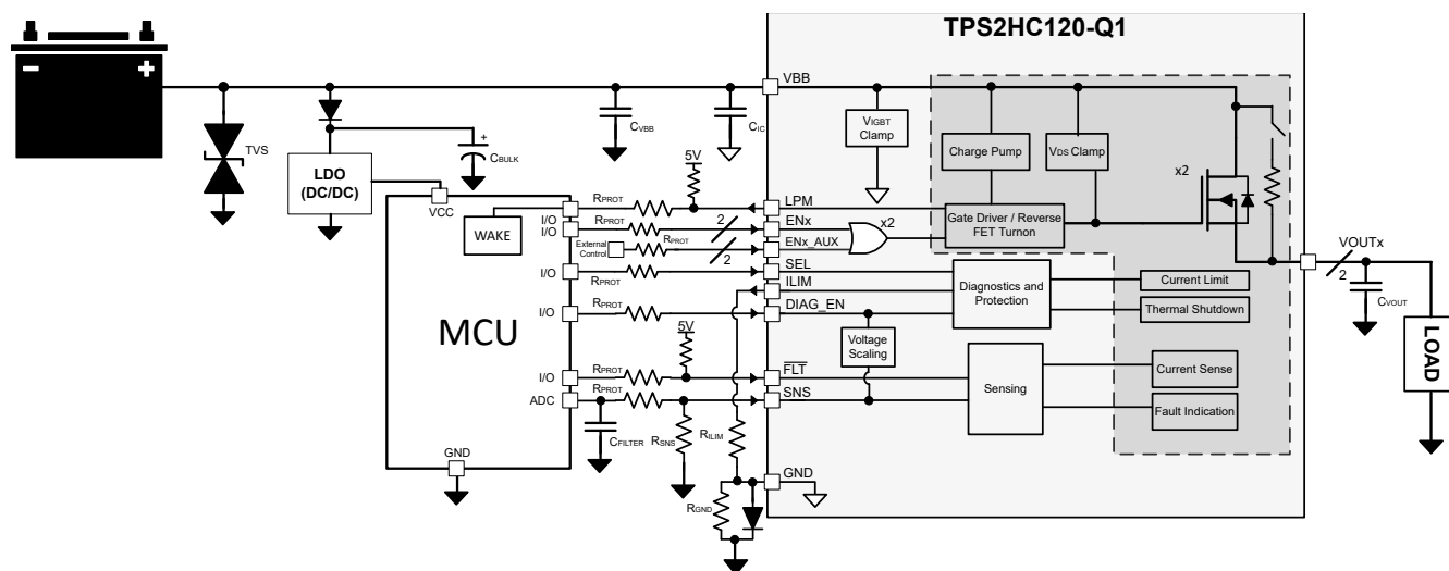
Figure 8-1. Typical Application Diagram
