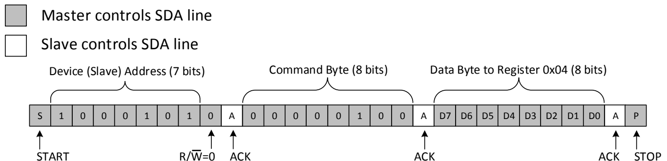
Figure 15. Write to the Fully On Register (0x04)
