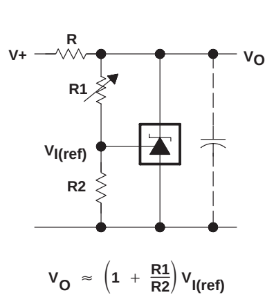
Figure 5. Shunt Regulator
