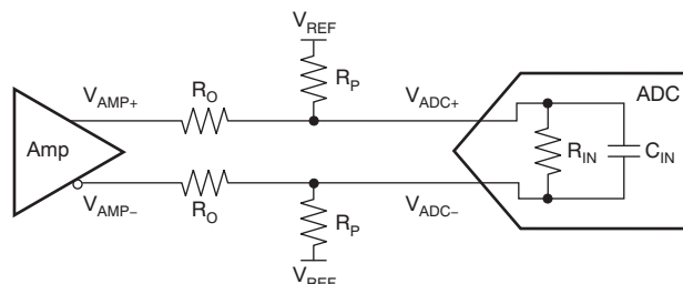
Figure 41. Resistor Network to DC Level Shift Common-Mode Voltage
