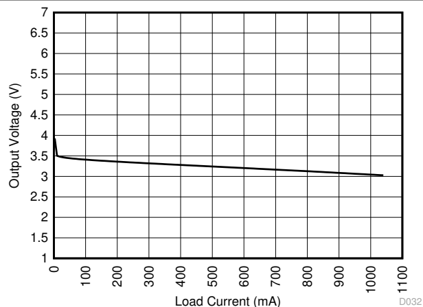
Figure 6-7. Output Voltage vs Load Current
