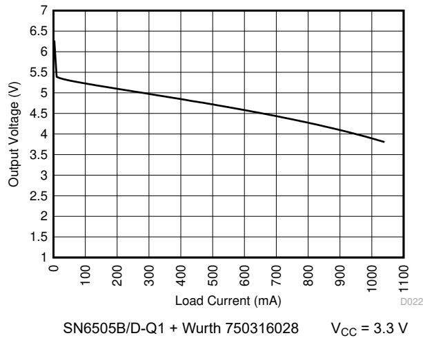
Figure 6-25. Output Voltage vs Load Current
