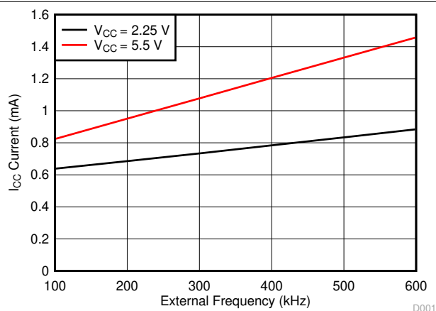
Figure 6-10. Current vs External Frequency
