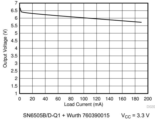
Figure 6-23. Output Voltage vs Load Current
