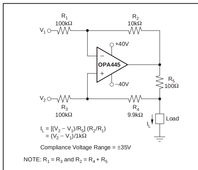
Figure 15. Voltage-to-Current Converter
