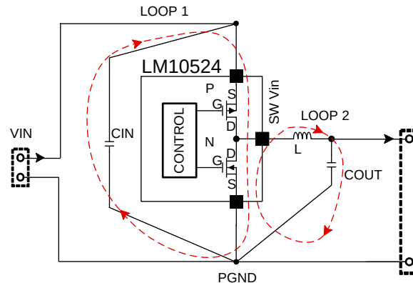
Figure 29. Buck Schematic Showing Layout Sensitive Nodes
