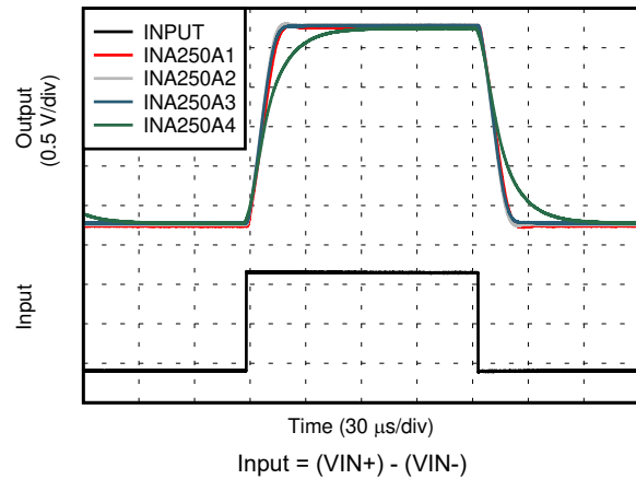
Figure 6-27. Step Response
