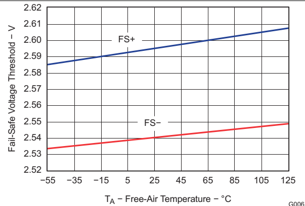
Figure 8. Fail-safe Voltage Threshold Vs Free-air Temperature
