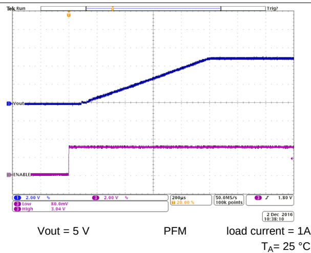
Figure 56. Start-Up Timing
