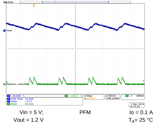
Figure 36. Output Voltage Ripple
