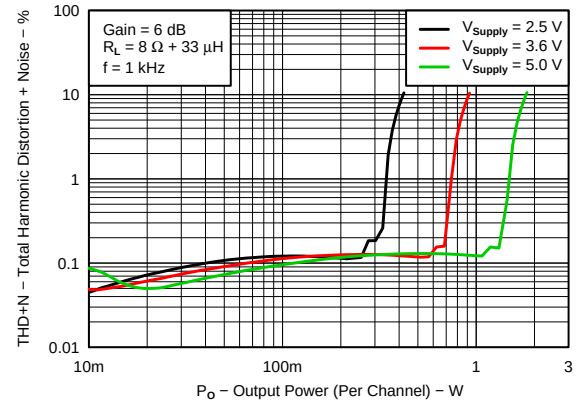
Figure 18. Total Harmonic Distortion + Noise vs Power, 8 \Omega
