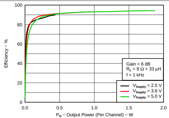
Figure 20. Efficiency vs Output Power (Per Channel), 8 \Omega
