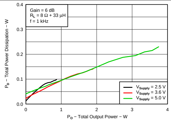
Figure 22. Total Power Dissipation vs Total Output Power, 8 \Omega
