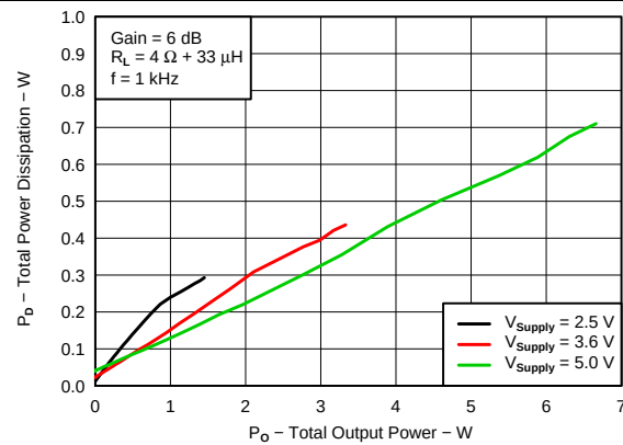
Figure 21. Total Power Dissipation vs Total Output Power, 4 \Omega
