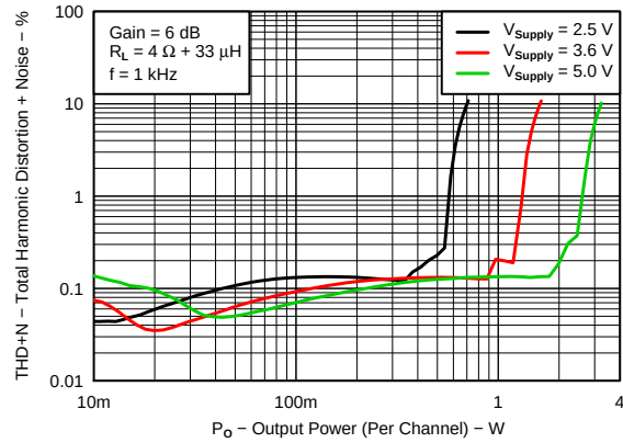
Figure 17. Total Harmonic Distortion + Noise vs Power, 4 \Omega
