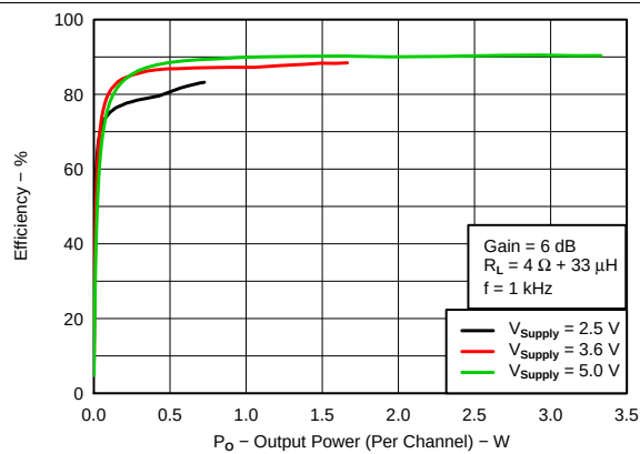
Figure 19. Efficiency vs Output Power (Per Channel), 4 \Omega
