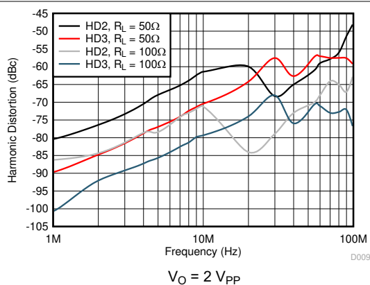
Figure 5-17. Harmonic Distortion vs Frequency
