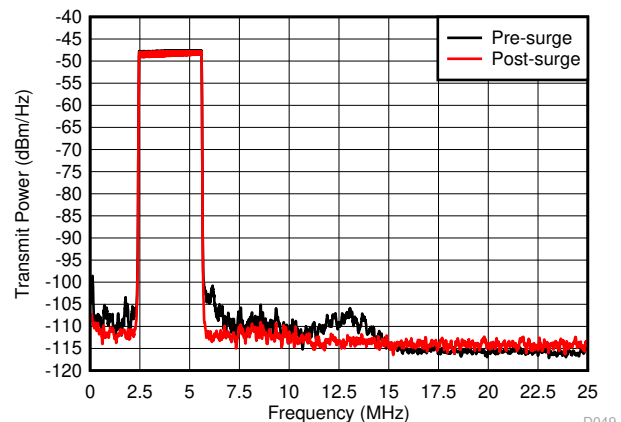
Figure 6-9. China SGCC HPLC Band1 Pre-Surge and Post-Surge
