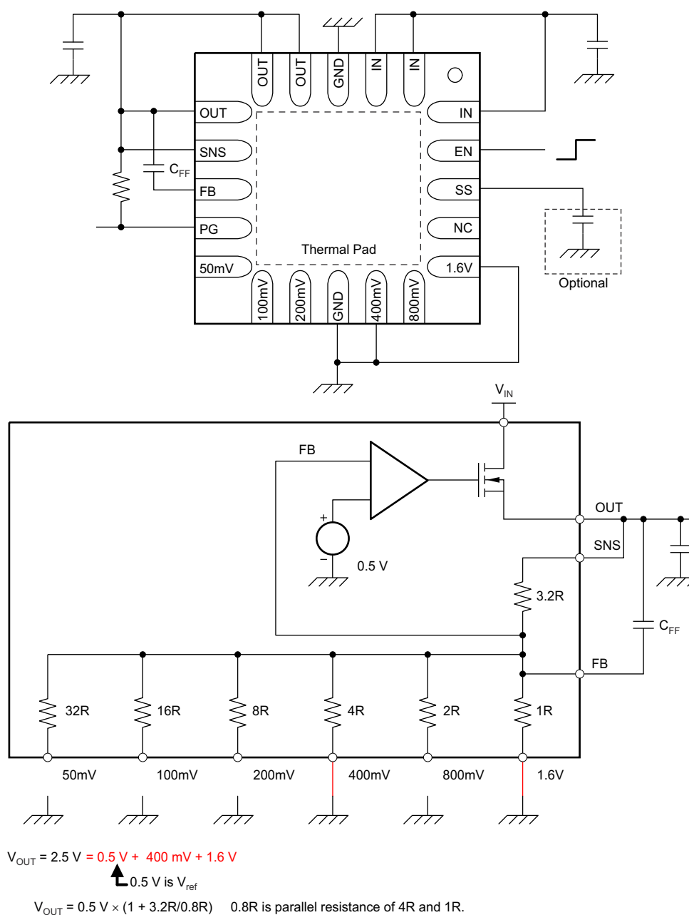
Figure 6-4. 2.5-V Configuration
