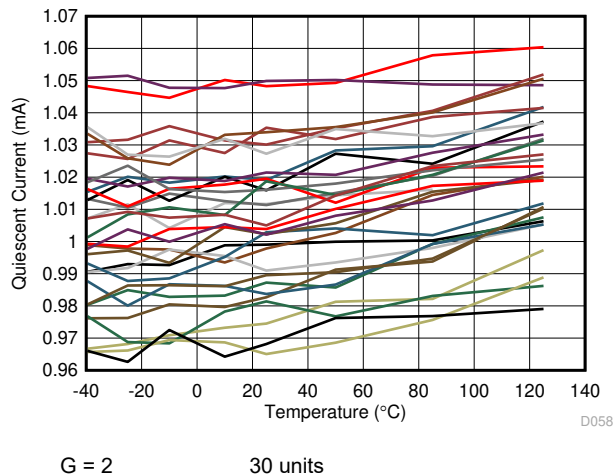
Figure 7-58. Supply Current vs Temperature
