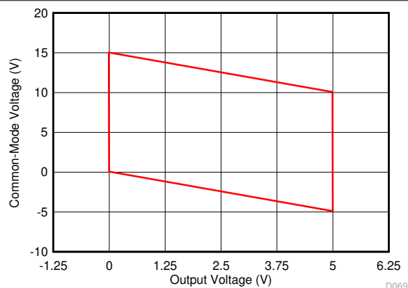
G = 1/2 5-V supply V_{REF} = 0\text{ V}
