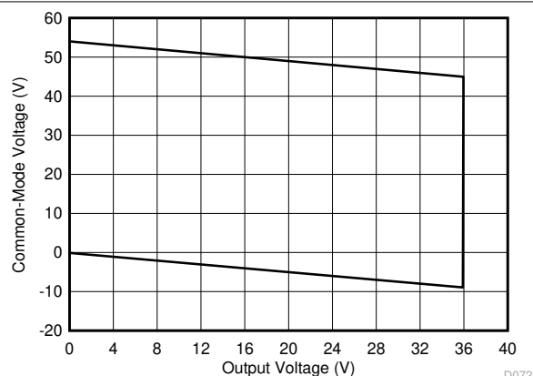
G = 2 36-V supply V_{REF} = 0\text{ V}
