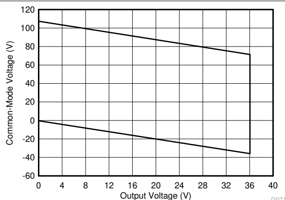
G = 1/2 36-V supply V_{REF} = 0\text{ V}
