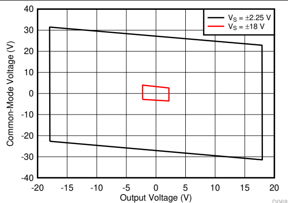
G = 2 Bipolar supply V_{REF} = 0\text{ V}
