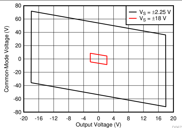
G = 1/2 Bipolar supply V_{REF} = 0\text{ V}
