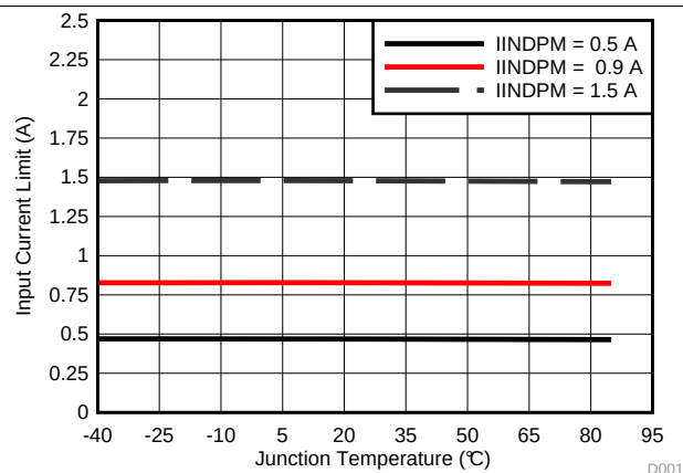
Figure 5. Input Current Limit vs. Junction Temperature
