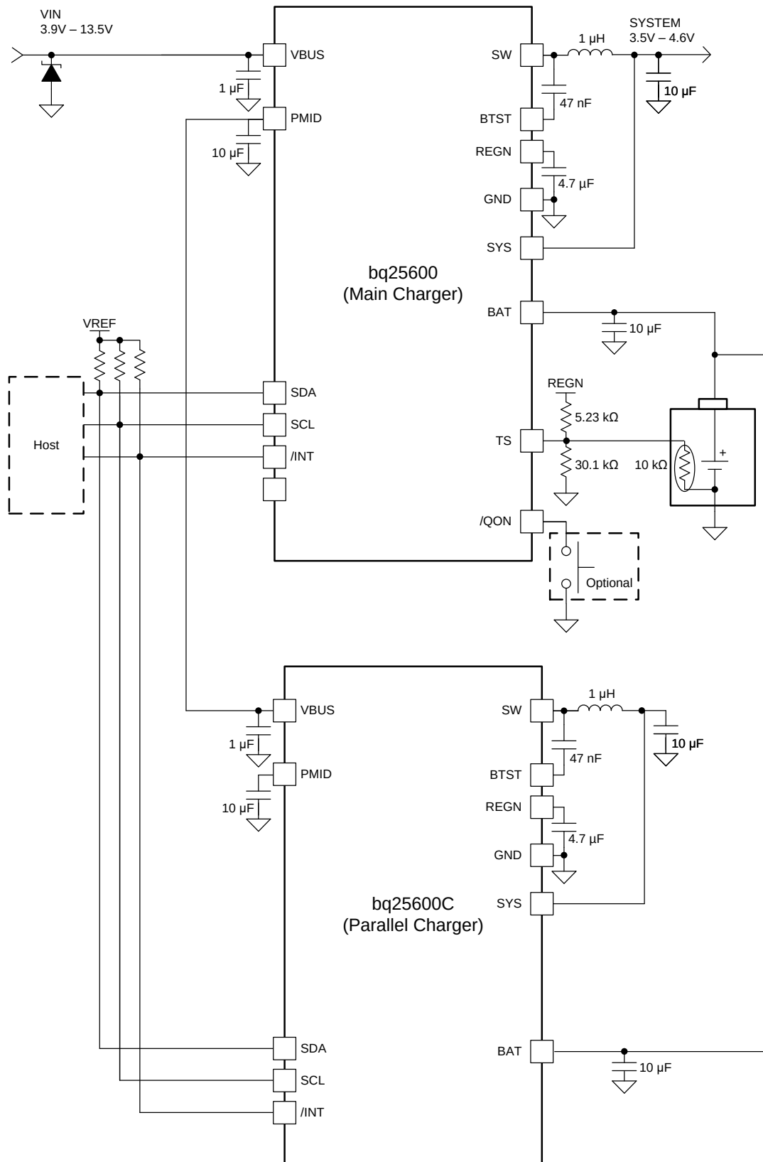
Figure 19. Parallel Charger Application
