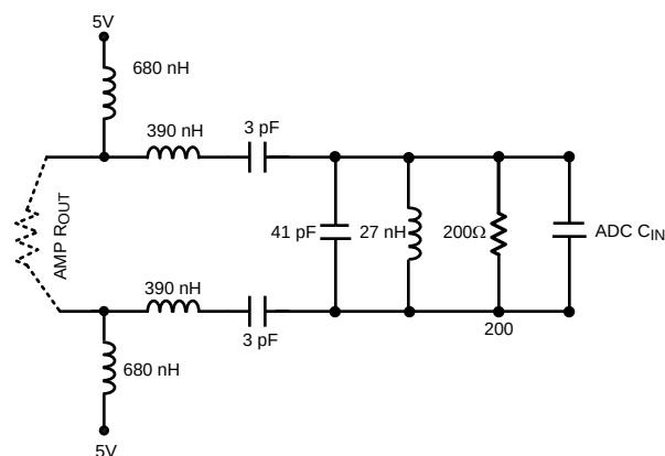
Figure 44. Bandpass Filter Center Frequency is 140 MHz with a 20 MHz Bandwidth Designed for 200Ω Impedance
