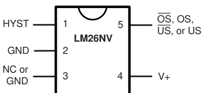
Figure 4-1. 5-Lead SOT-23 See DBV Package
