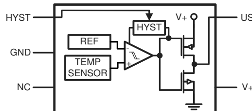
Figure 6-3. LM26CIM5 - __ F
