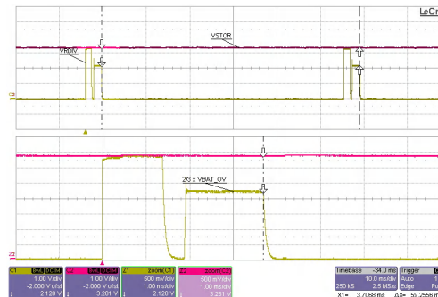
Figure 9-17. Boost Charger Operational Waveforms
