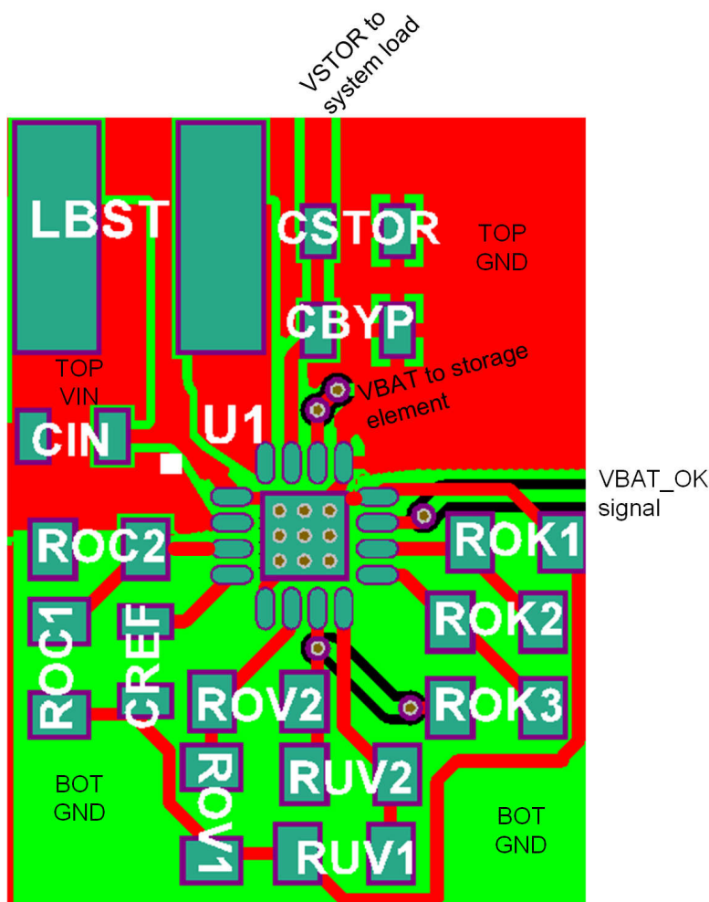
Figure 11-1. Recommended Layout
