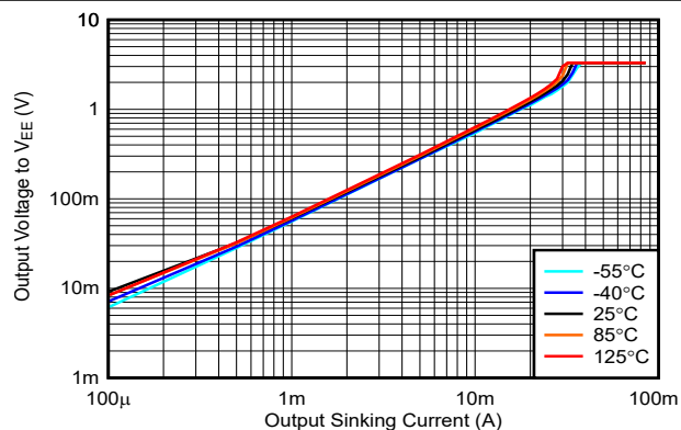
Figure 5-20. Output Voltage vs. Output Sinking Current, 3.3V
