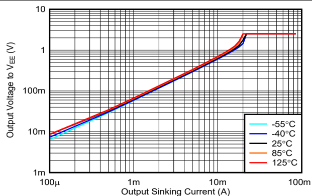
Figure 5-18. Output Voltage vs. Output Sinking Current, 2.5V
