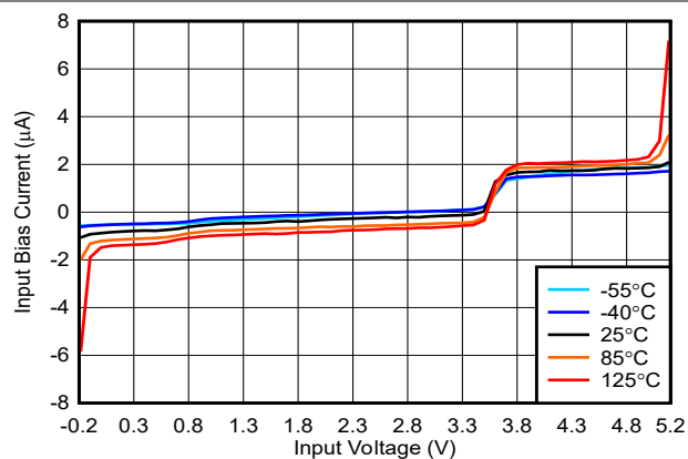
Figure 5-16. Bias Current vs. Input Voltage, 5V
