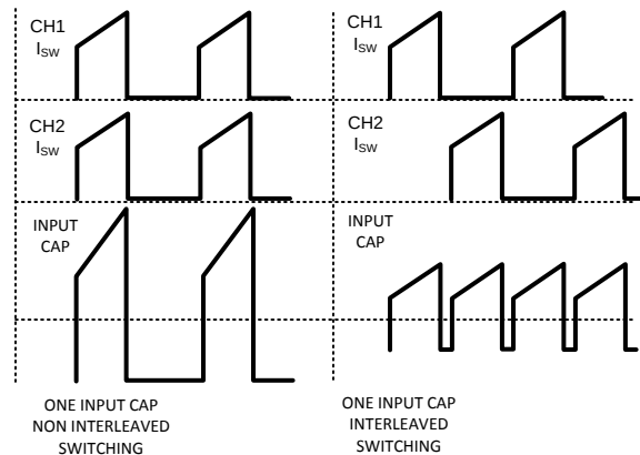
Figure 20. Switch and Input Capacitor Currents
