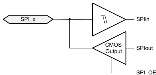
Figure 9-50. IOBUF_GPIOHSSI
