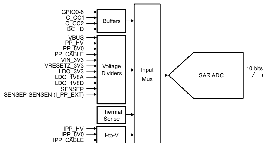
Figure 9-44. SAR ADC
