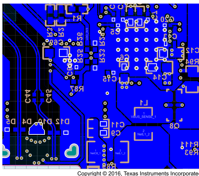
Figure 12-11. Bottom Layer Component Routing
