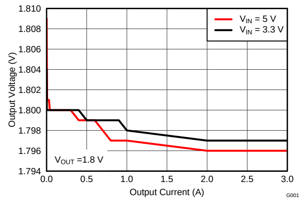
Figure 4. DC Load Regulation
