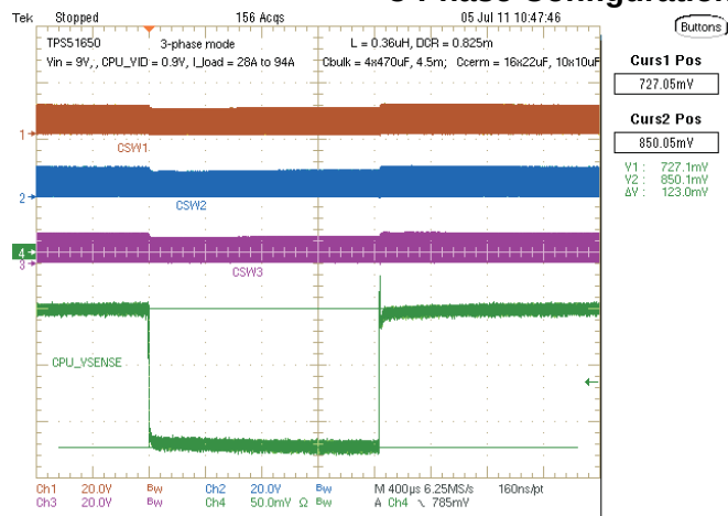
Figure 7. Load Transient: V_{IN} = 9\text{ V} , Load-step = 66 A
