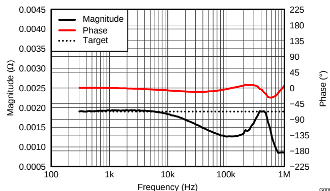
Figure 18. Output Impedance
