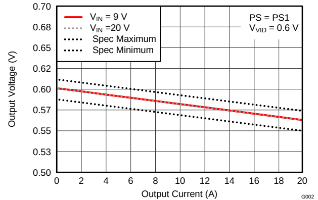
Figure 2. Output Voltage vs. Load Current in PS1
