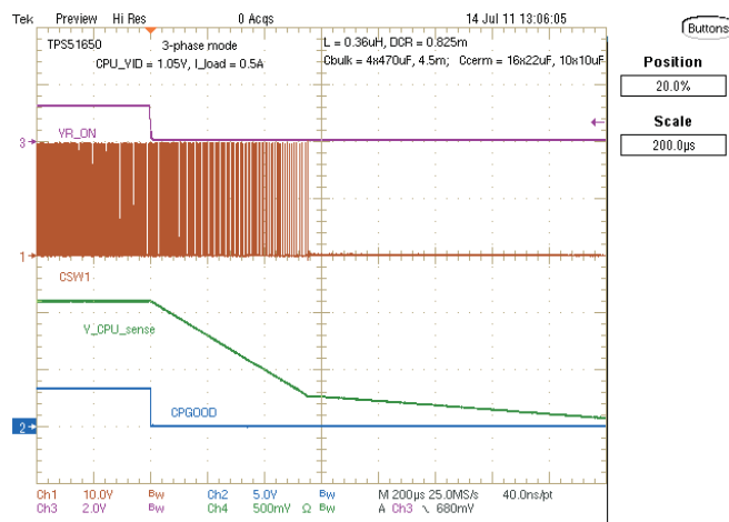
Figure 12. Soft-Stop
