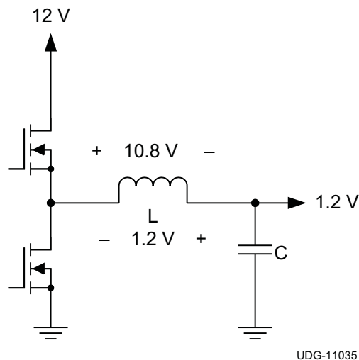
Figure 45. Synchronous Converter
