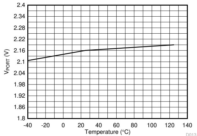
Figure 7-13. Power Good Threshold vs Temperature
