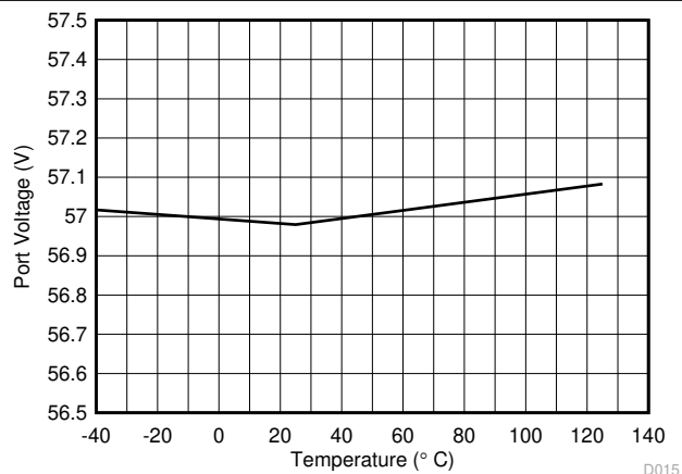
Figure 7-15. Port Voltage ADC Measurement vs Temperature
