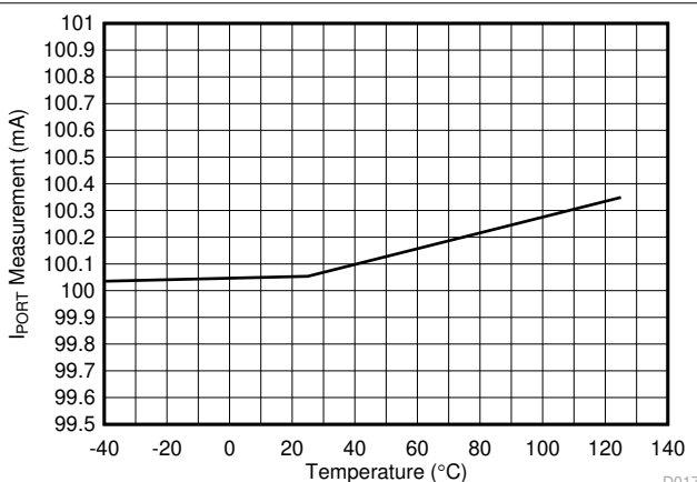
Figure 7-17. Port Current ADC Measurement (100mA) vs Temperature
