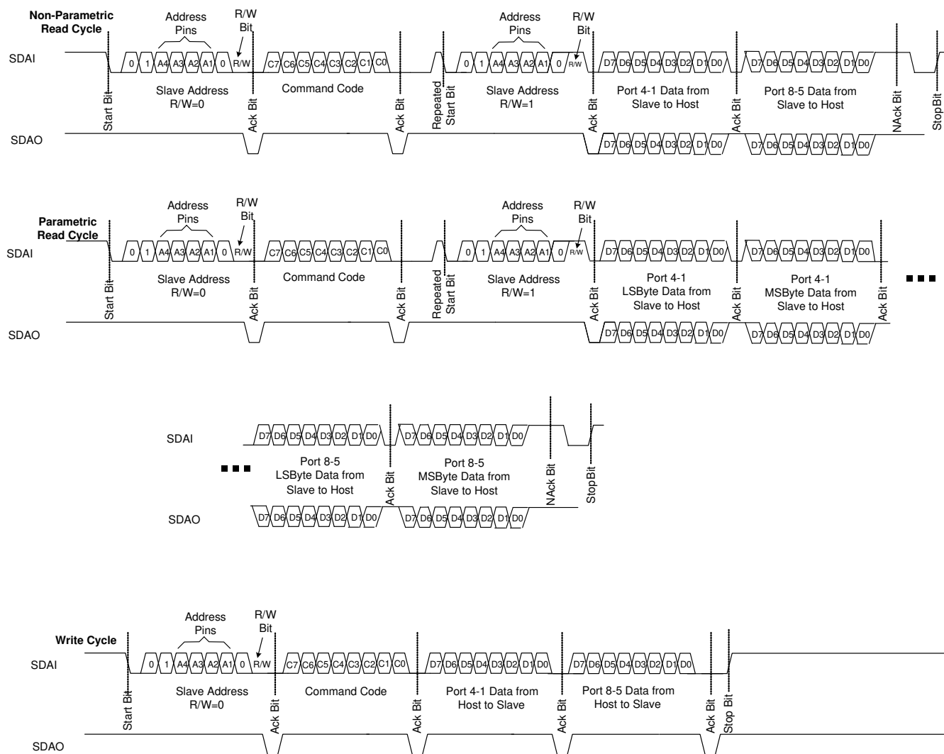
Figure 9-5. I 2 C interface Read and Write Protocol – Configuration B
