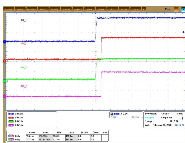
V_{CC} = 5\text{ V} R_L = 60\ \Omega Figure 9-5. t_{PROP(LOOP2)} Transceiver 1 & Transceiver 2
