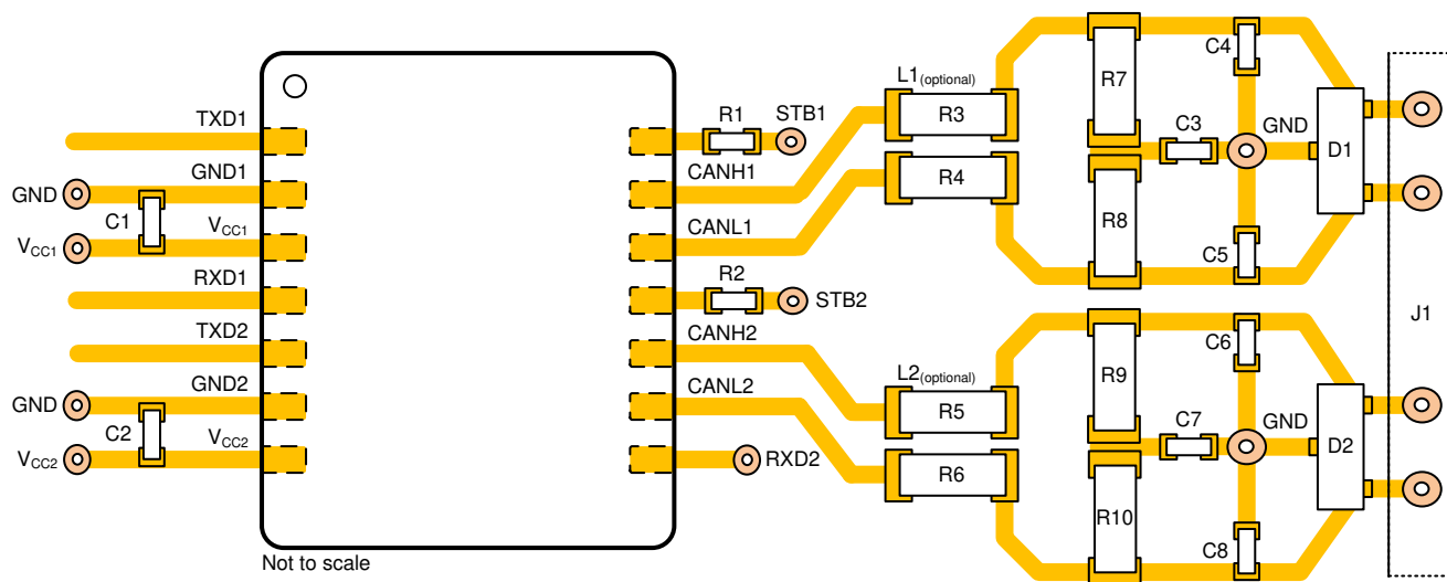
Figure 11-1. Layout Example
