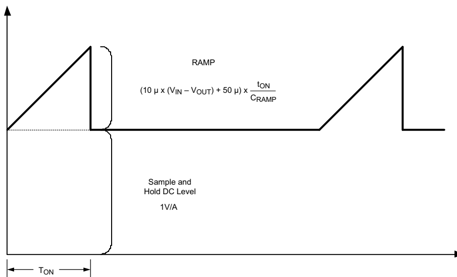
Figure 8. Composition of Current Sense Signal
