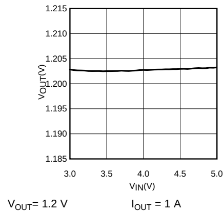
Figure 14. Buck 3 V_{OUT} vs V_{IN}
