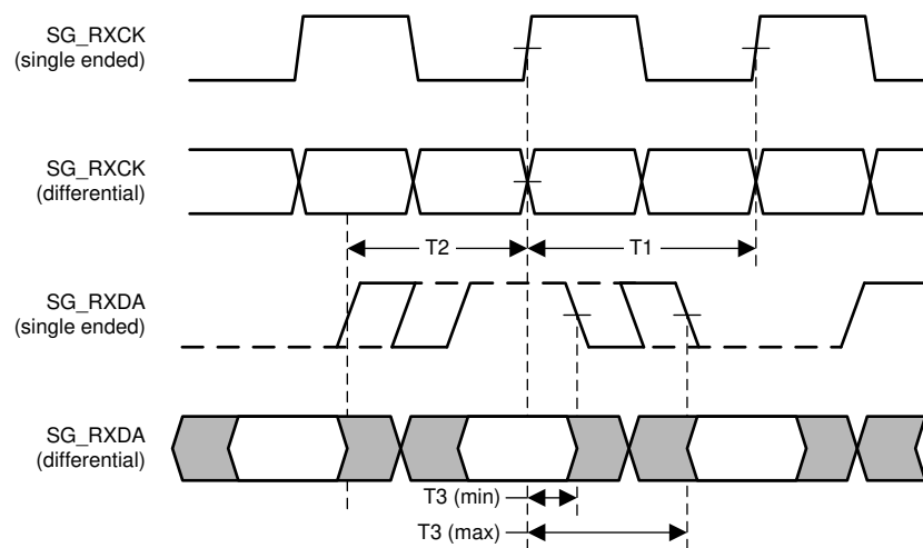
Figure 6-4. SGMII Timing
