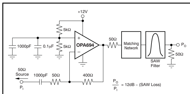
Figure 35. IF Amplifier Driving SAW Filter
