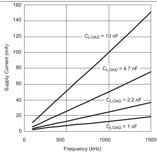
Figure 5. Supply Current vs Frequency ( V_{DD} = 5 V)
