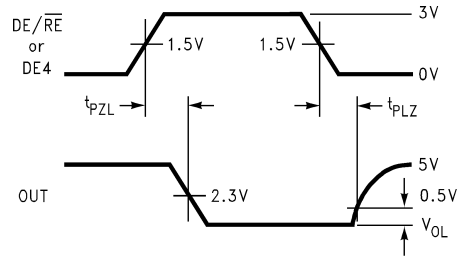
Figure 8. Driver Enable and Disable Timing ( t_{PZL} , t_{PLZ} )
