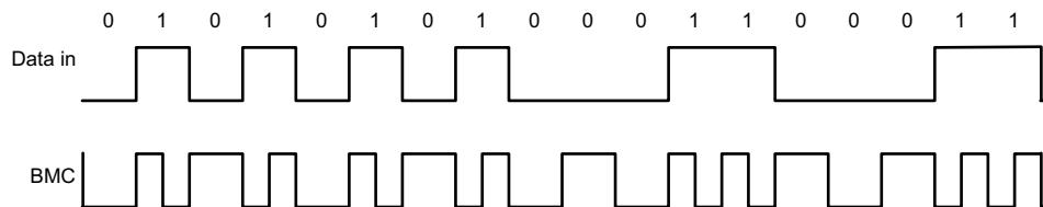
Figure 8-6. Biphase Mark Coding Example
